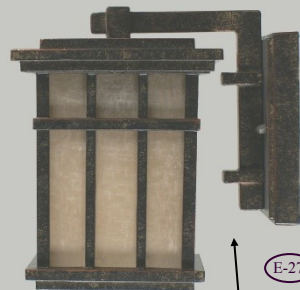
E-27 QUADRANT SMALL EXT W/B BRONZE FRAME SIZE H - 25cm W - 16cm P - 22cm
