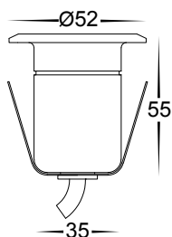
Cutout without Canister — Ø38 —
