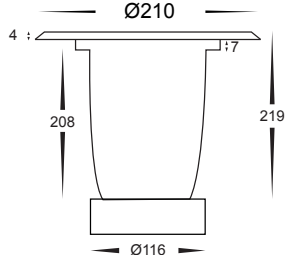
Cutout without Canister Ø182 Ø210
