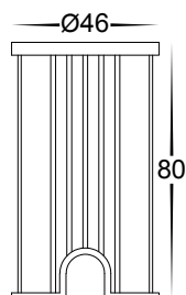
Cutout with Canister — Ø46 —
