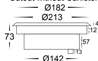
Cutout without Canister
