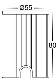
Cutout with Canister — Ø55 —
