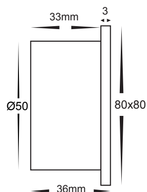
Cutout without Canister Ø60
