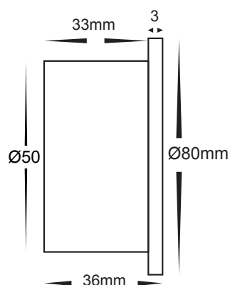
Cutout without Canister Ø60
