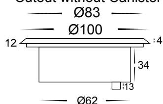
Cutout without Canister
