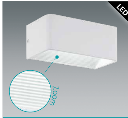
96205 SANIA 3 wall luminaire; aluminium, white
