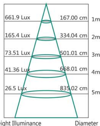
Lux Distance Curve
