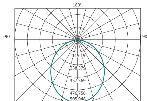
Polar Curve
