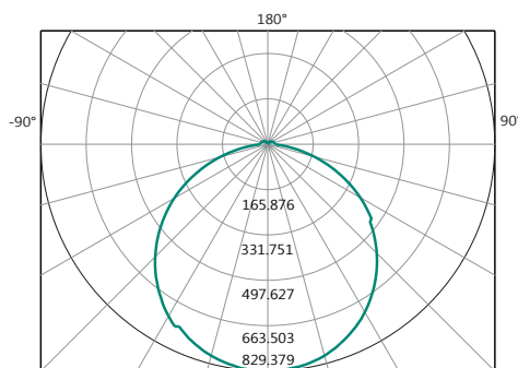
Polar Curve
