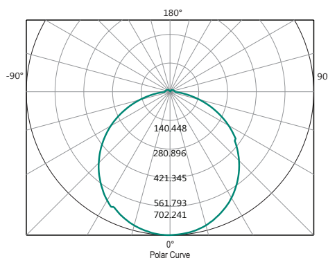
Polar Curve
