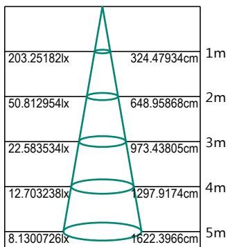
Lux-Distance Diagram
