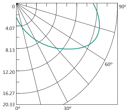
Light Distribution Curve (Unit: cd)
