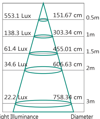
Lux Distance Curve
