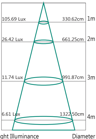
Lux Distance Curve
