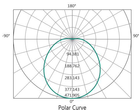
Polar Curve
