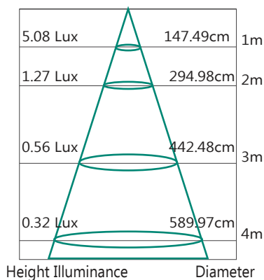
Lux Distance Curve
