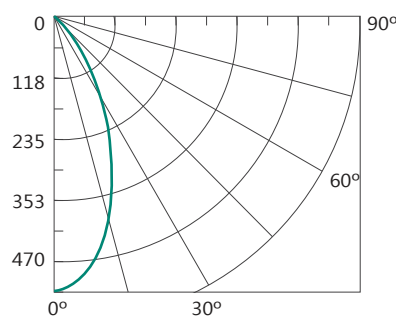
Light Distribution Curve (Unit: cd)
