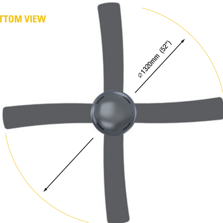
Dimensions of fan with Light Kit
