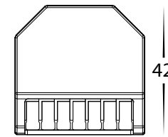
HV9271 Dimensions
