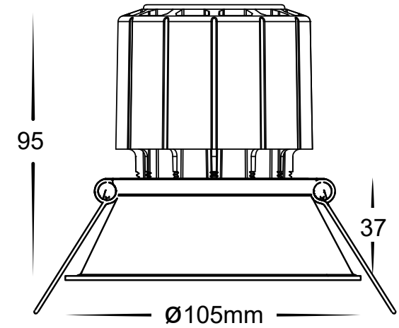
Installation Diagram
