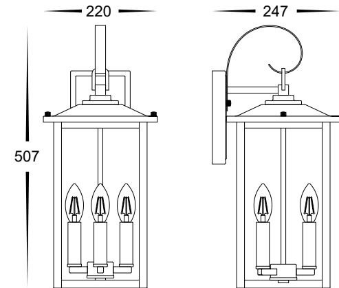
HV3535W-M-BLK Dimensions
