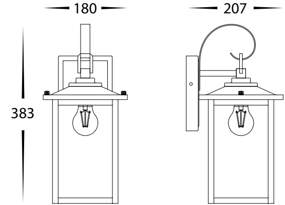
HV3535W-M-BLK Dimensions
