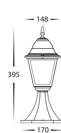
HV1651W-BLK Dimensions
