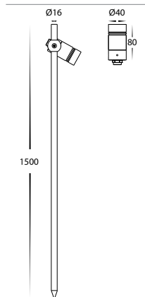
HV1441T-2-BLK Dimensions
