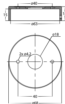
Mounting Base
