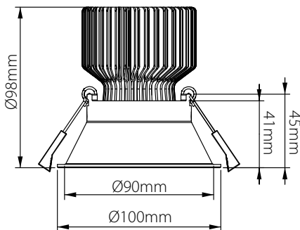
Cutout: Ø90mm
