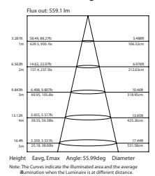
Beam diagram
