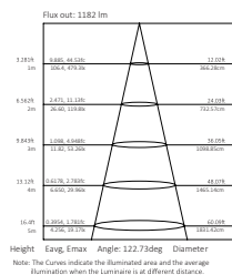
Beam diagram
