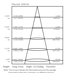
Beam diagram
