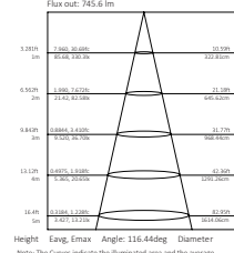
Beam diagram
