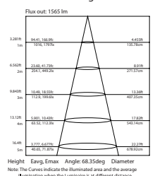
Beam diagram
