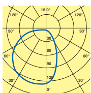
Cod. 9010 — piano verticale vertical plane
