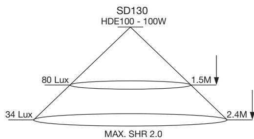
Double Envelope Halogen Superlux HDE-100-E27
