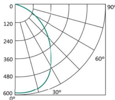
Light Distribution Curve (Unit: cd)
