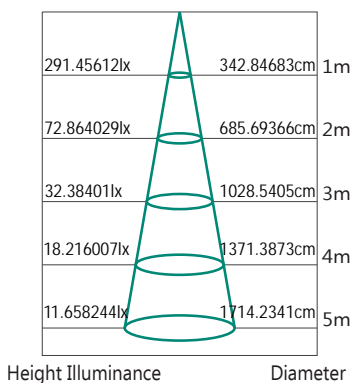
Lux Distance Curve
