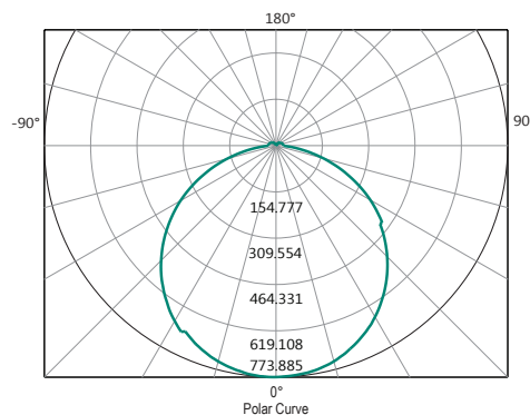
Polar Curve
