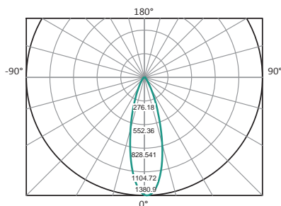
Polar Curve
