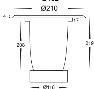
Cutout without Canister Ø182
