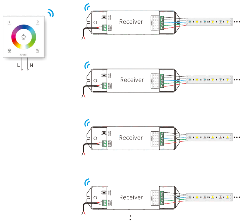
Sample wiring diagram
