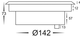
Cutout without Canister Ø182 Ø213
