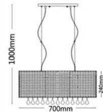
GEM6-O Oval Black 4xE14 Iron/PVC shade/ Crystal L : 700mm W: 250mm H : 1000mm
