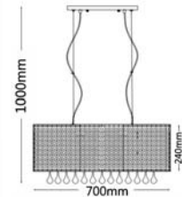
GEM5-O Oval Silver 4xE14 Iron/PVC shade/ Crystal L : 700mm W: 250mm H : 1000mm
