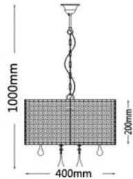
GEM1-R Round Brown 3xE14 Iron/PVC shade/ Crystal D: 400mm H: 1000mm
