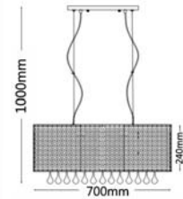
GEM4-O Oval Brown 4xE14 Iron/PVC shade/ Crystal L : 700mm W: 250mm H : 1000mm
