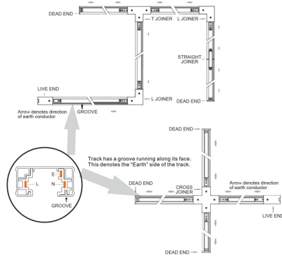
SINGLE CIRCUIT TRACK DIAGRAM
