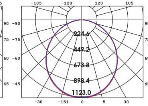
SL2110/50CW at 4000K
