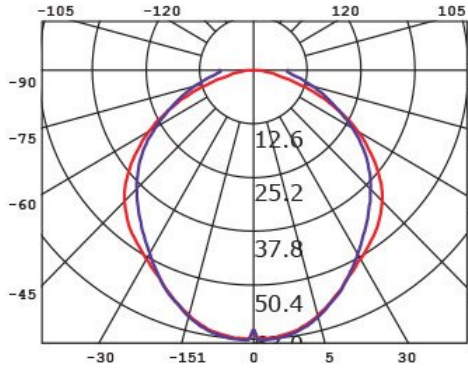
SL2110/10CW at 4000K
