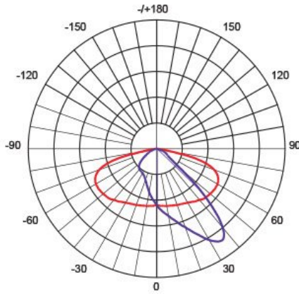
SHP305/180NDL at 5000K with SHP305A45/P
