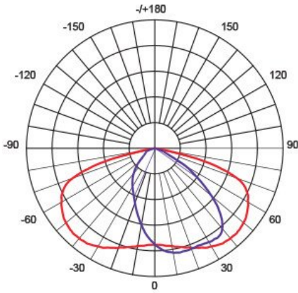
SHP305/70NDL at 5000K with SHP305A75/P
