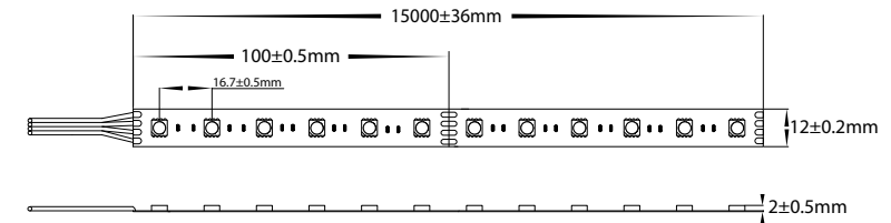
IP54 12mm (W) x 3mm (H) LED Strip Dimensions
