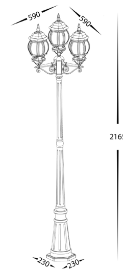
HV1673 Dimensions
