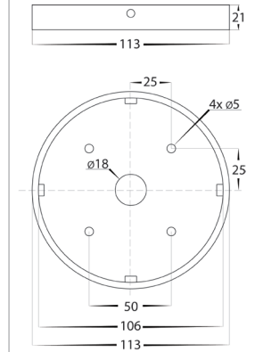
Mounting Bracket
