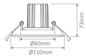
Cutout: Ø80-85mm
