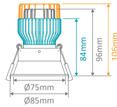
Cutout: Ø75-77mm
