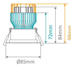
Cutout: Ø70-75mm
