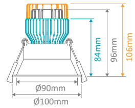
Cutout: Ø90-92mm DT90 Tiltable to 15°
