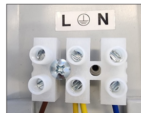
Terminal block: PA14, 500V, VDE
