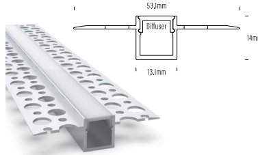
AQS-EXT-011 Aluminium / White 14mm H x 35.9mm W x 2m L
