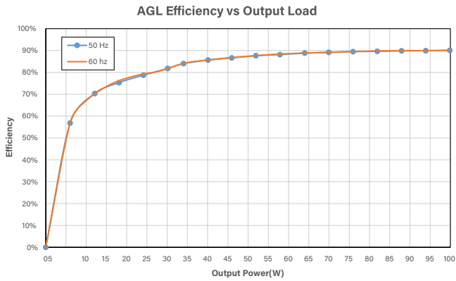
Power supply had achieved >70% efficiency for as low as 12W output load.
