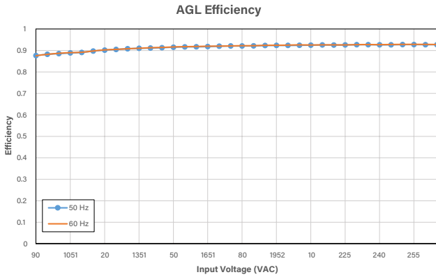
Power supply had >86% efficiency across whole input range.
