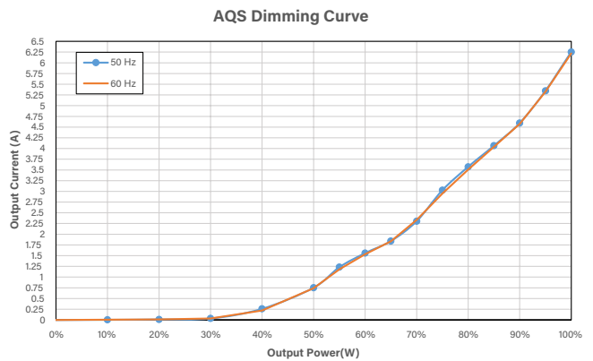
Test confirmed no flickering and shimmering from 0 to 100% on 150W AQS.
