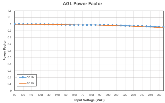
Power supply had >95 PF across whole input range.
