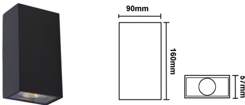
STELLAR Rectangle up & down wall light
