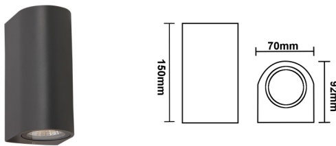
ERIS Round black up and down wall light
