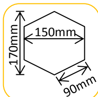
Base Dimensions
