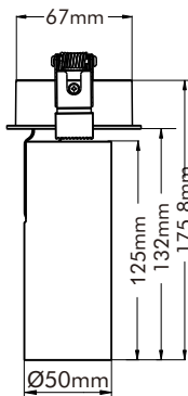
Cut out: Ø68mm
